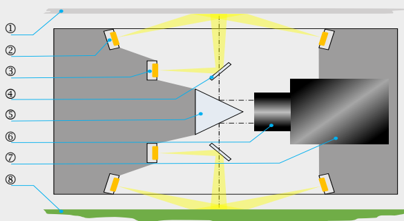
Schematic of the LIST camera
